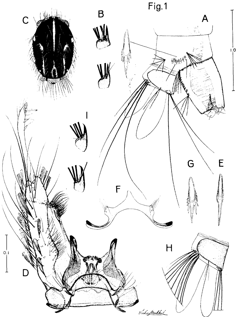
Fig. 1. A-D, Aedes (Stegomyia) seatoi n. sp.: A, lateral aspect of the terminal segments of the fourth instar larva with enlarged comb scale; B, meso- and metapleural spines of the larva; C, dorsal aspect of the holotype thorax; D, tergal aspect of the holotype terminalia. E-F, A. (S.) albopictus (Skuse): E, comb scale of the larva; F, tergum IX of the male terminalia. G-I, A. (S.) aegypti (L.): G, comb scale of the larva; H, ventral brush of the larva; I, meso- and metapleural spines of the larva.
