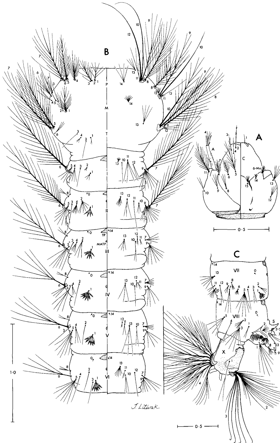
Fig. 2. Fourth-instar larva of Anopheles (Cellia) ainshansi . A, Head, dorsal (left) and ventral (right) aspects of left side. B, Thorax and abdominal segments I-VI, dorsal (left) and ventral (right) aspects of left side. C, Abdominal segments VII-X, left side. A, antenna; C, cranium; P, prothorax; M, mesothorax; MANP, median accessory tergal plate; S, spiracular lobe; T, metathorax; TP, tergal plate; I-VIII, X = abdominal segments I-VIII and X; 1-15 = setal numbers for specified areas, e.g., seta 5-C. Scales in mm.
